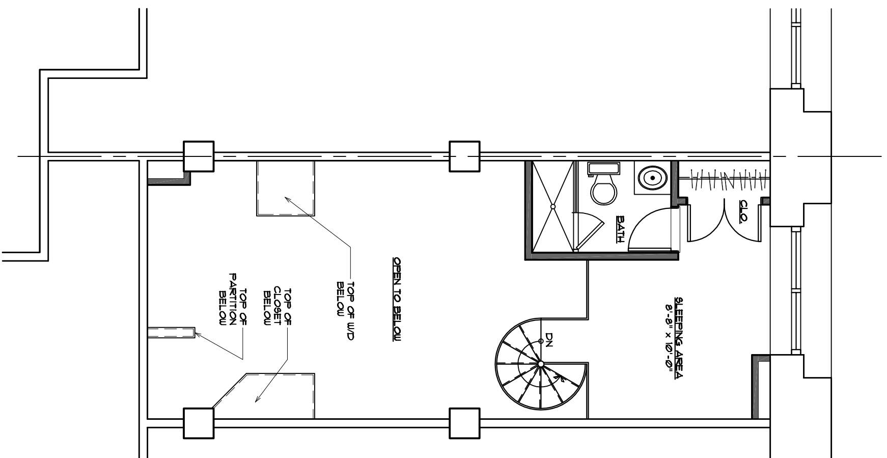
LOFT LEVEL PLAN (UNIT 102A) SCALE 3/16"=1'-0"
