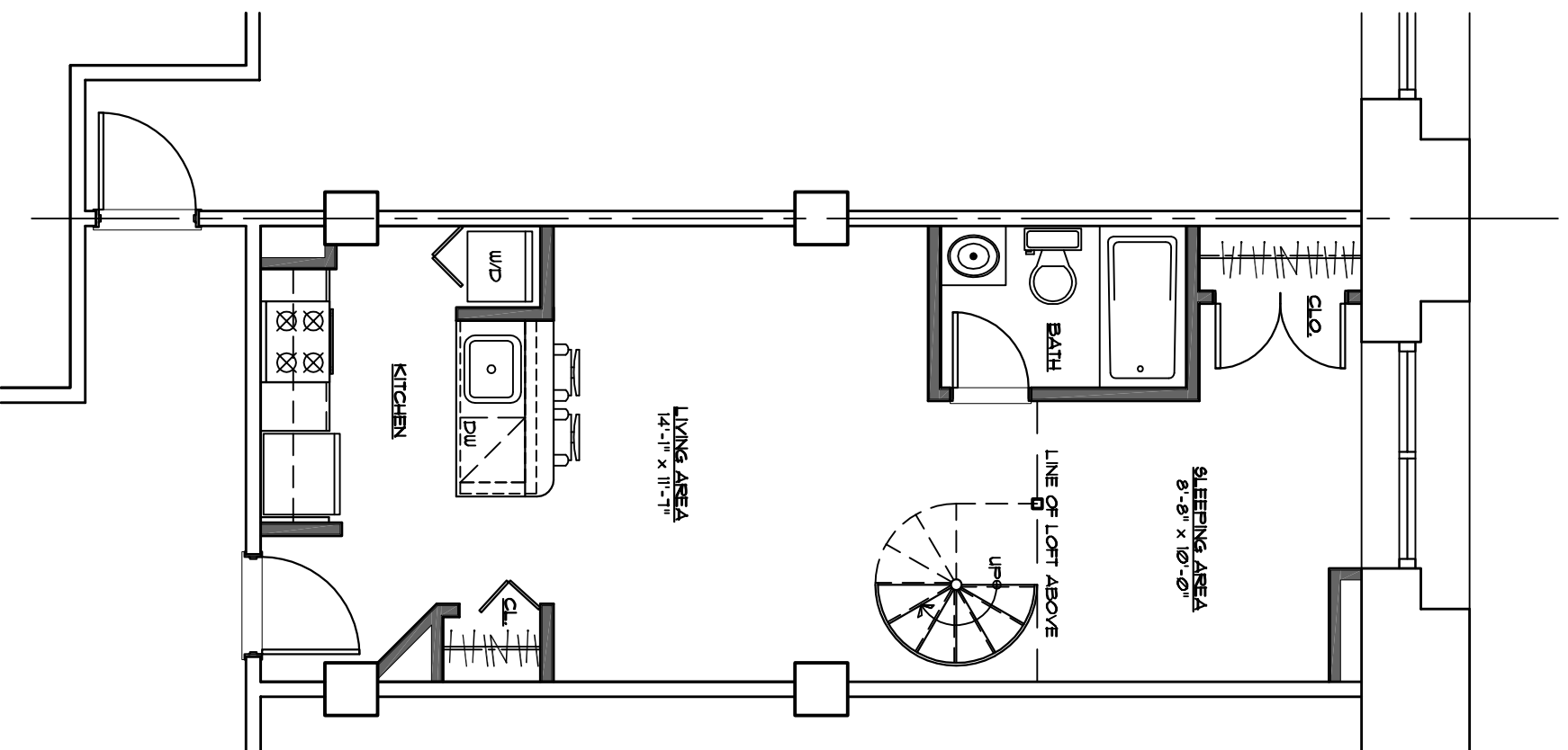
LOWER LEVEL PLAN (UNIT 102A) SCALE 3/16"=1'-0"
